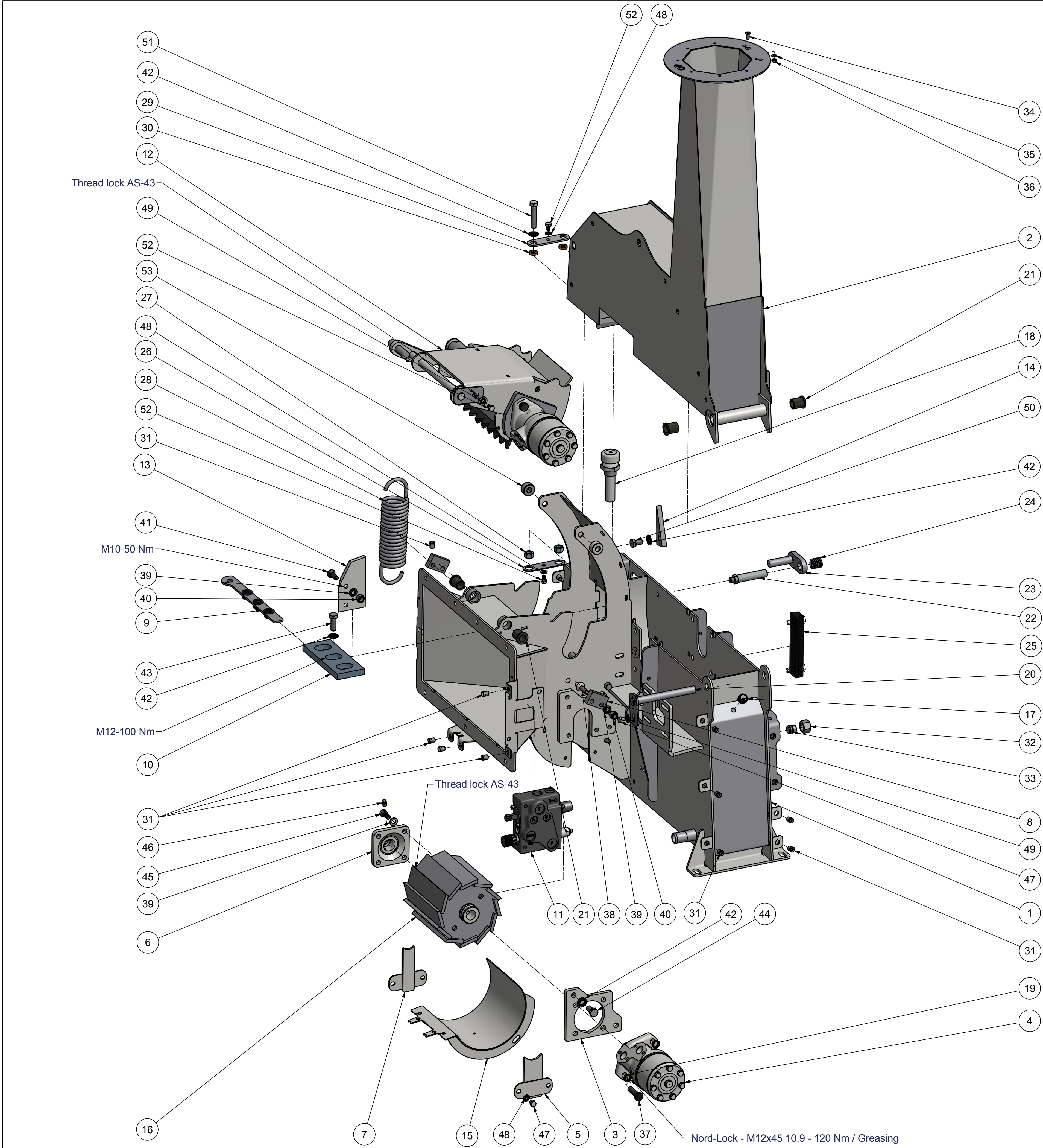
TP 175 MOBILE Spare parts list
