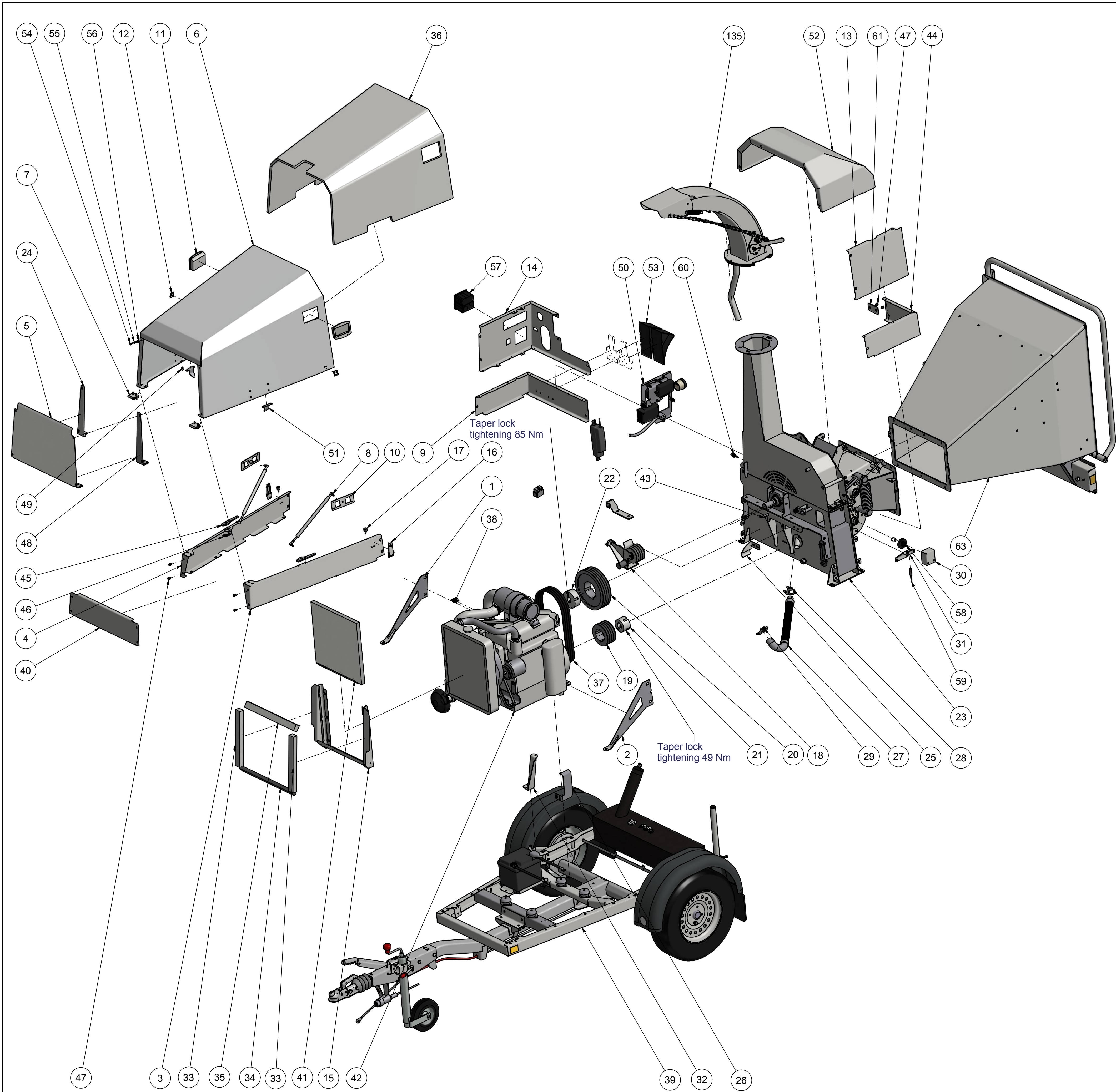
TP 175 MOBILE Spare parts list
