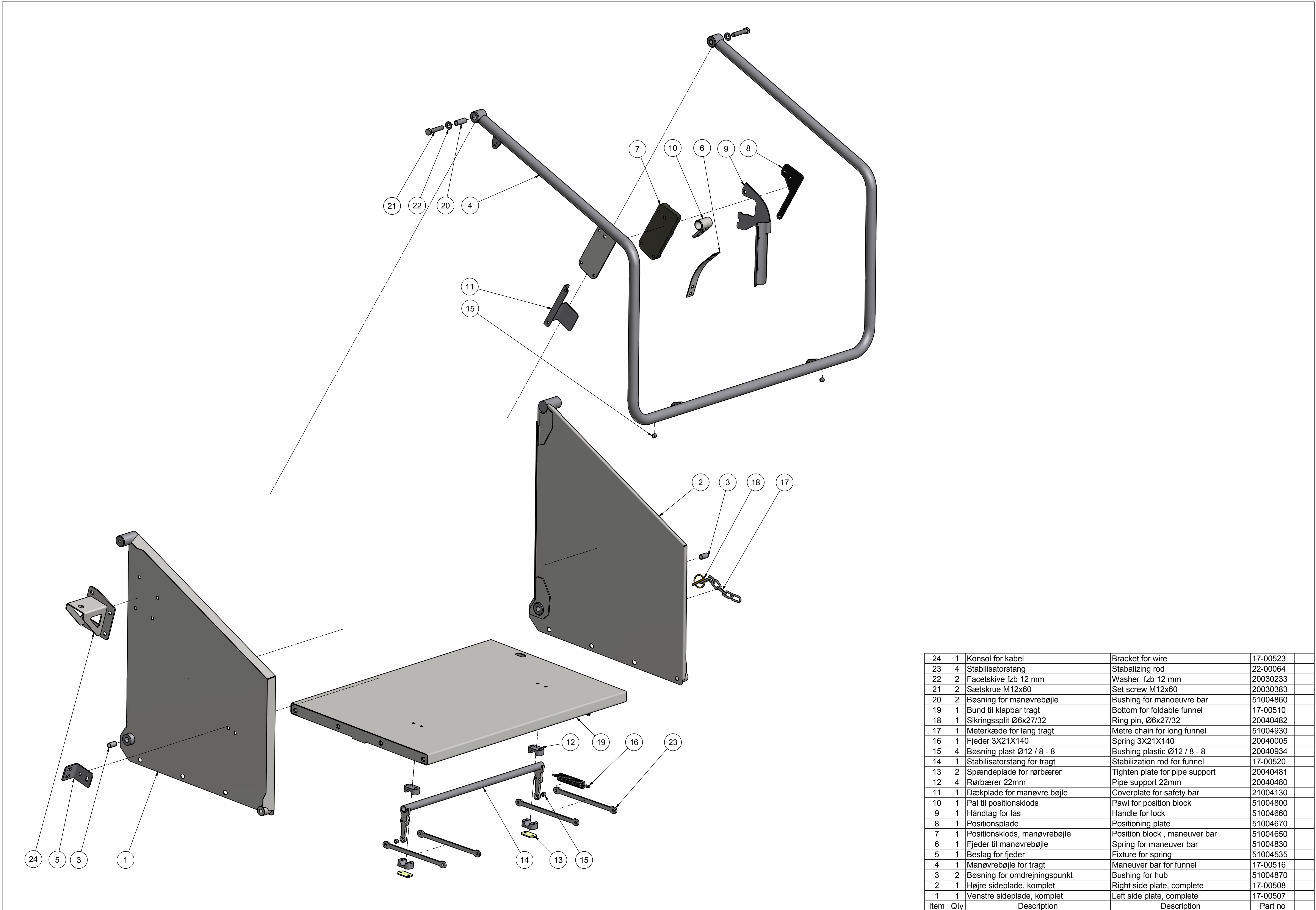
TP 175 MOBILE Spare parts list
